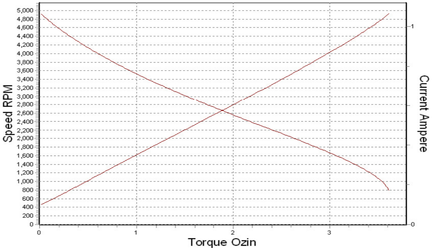
Torque Speed Torque Current
