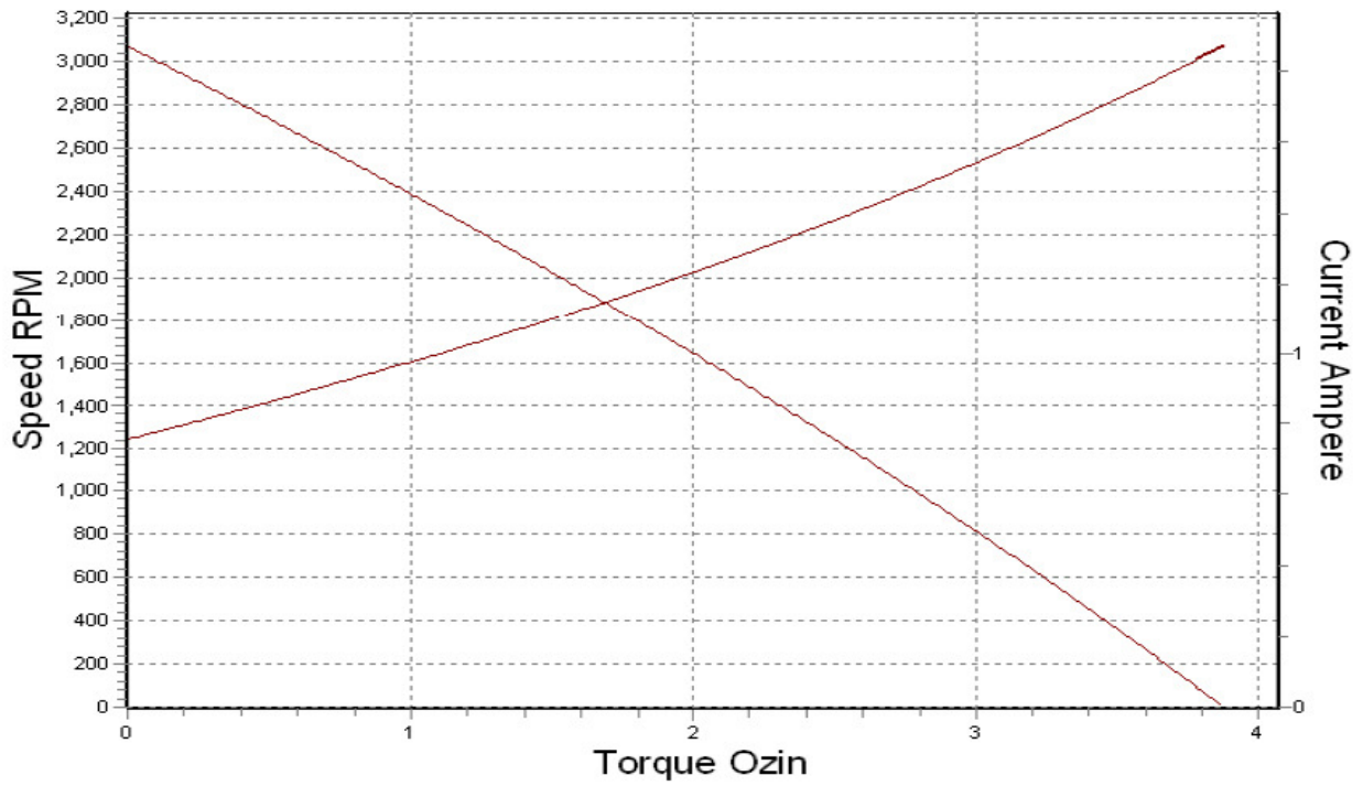
Torque Speed Torque Current
